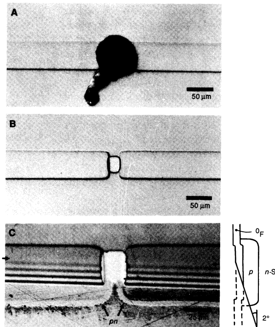
Fig. 2. Structure of the neuron-Si junction. (A) Top view of the FET with a Retzius cell. The horizontal band (width, 50 \mu\text{m} ) reflects source and drain. (B) Top view of the FET. The visible distance between source and drain is 16 \mu\text{m} . The contours mark the range of primary deposition of boron (groove of depth 150 nm), not the location of the pn junctions. In the center the insulating oxide (1 \mu\text{m} ) is opened over an area 22 \mu\text{m} by 30 \mu\text{m} . This region is covered by the gate oxide (thickness 20 nm). (C) The pn junctions. The lower half of the FET is ground at an angle of 2° up to the edge marked by the two arrows. The geometry is illustrated at the right (not scaled). The stripes are interference fringes due to the field oxide. The two pn junctions of source and drain—as stained by copper—are marked by arrows. Their horizontal distance at the gate is 6 \mu\text{m} .
